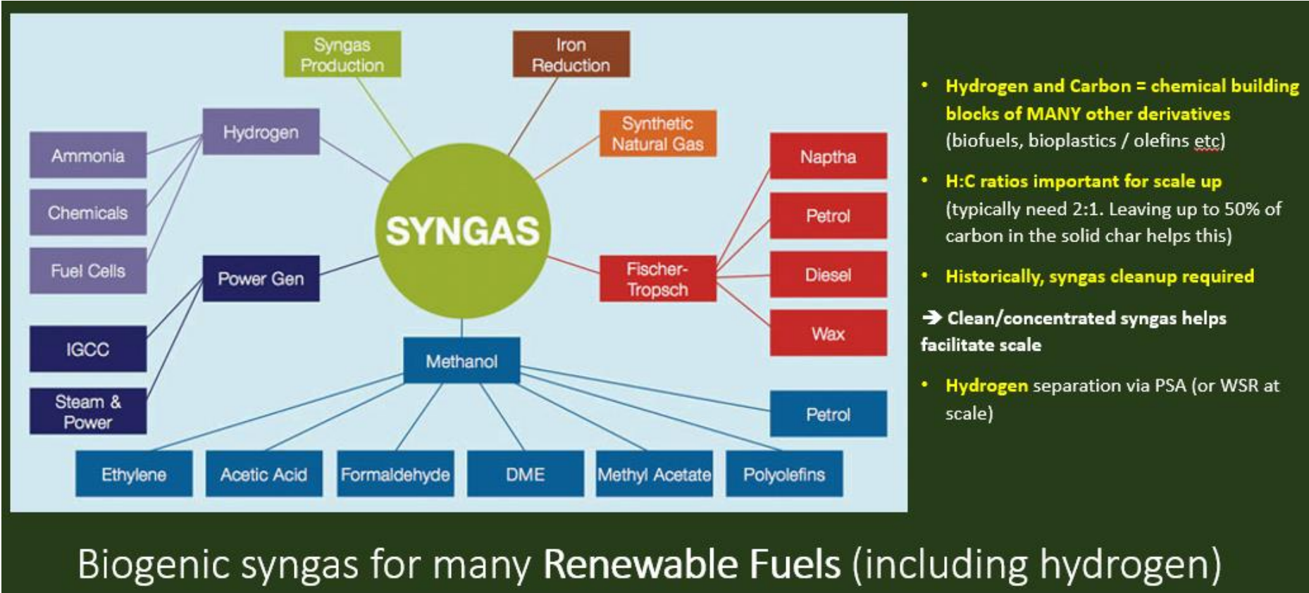
Figure 3: Syngas: Electricity and much more - Biogenic syngas for renewable fuels (including biohydrogen)
