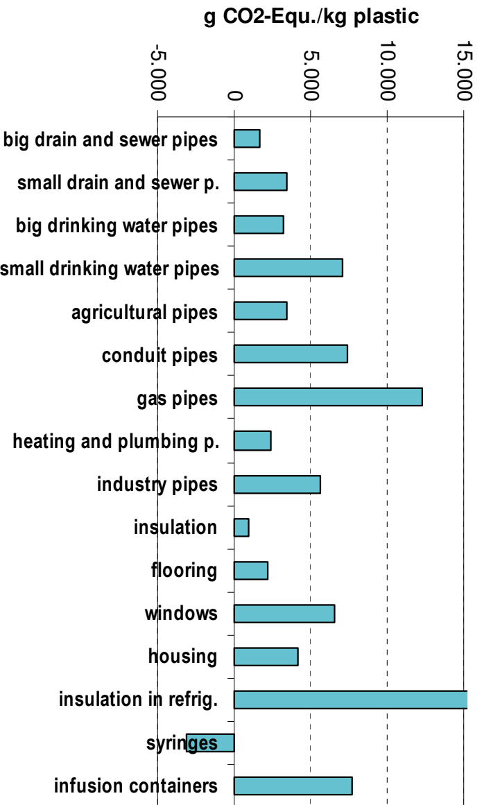
Figure 8: GHG emission savings of plastic products compared to alternative materials, given in gram (g) CO 2 -equivalent per kg plastic product. Figure shows second part of case studies. The value for “insulation in refrigerators” is approx. 79,000 g/kg PUR.
