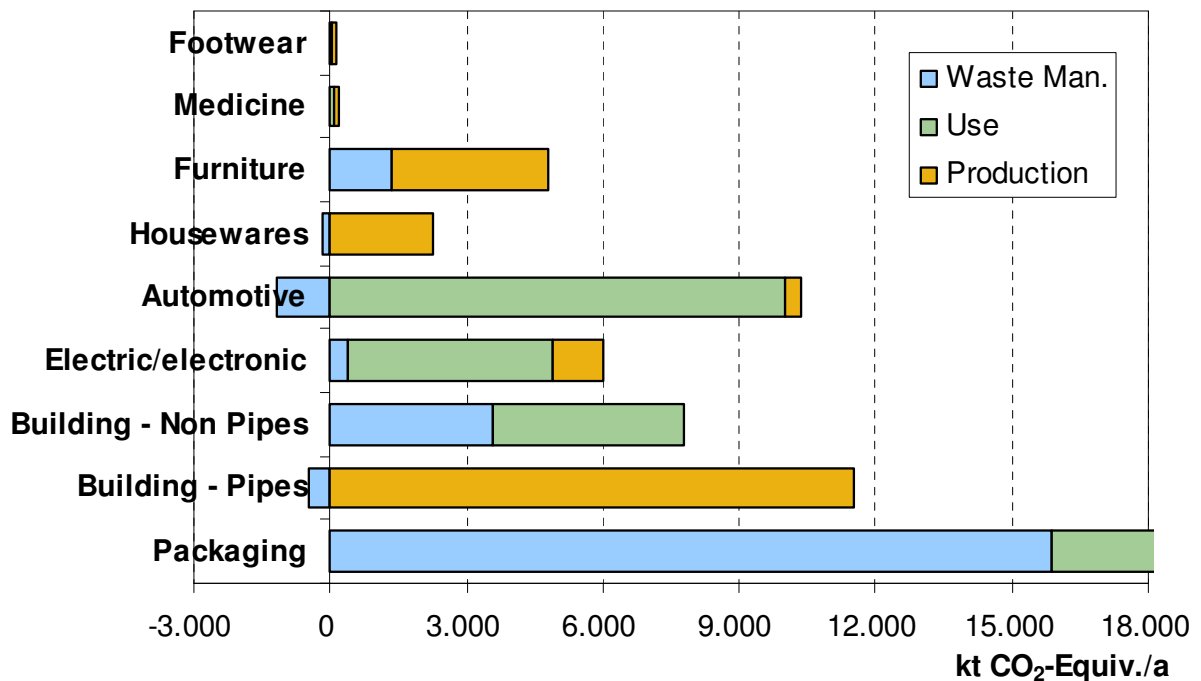
Figure 11: GHG emission savings (+) and additional GHG emissions (-) of plastic products compared to alternative materials, split into contributions of the life-cycle phases production, use and waste management. The total result for plastic packaging is 42.900 kt CO 2 -equivalents/a.
