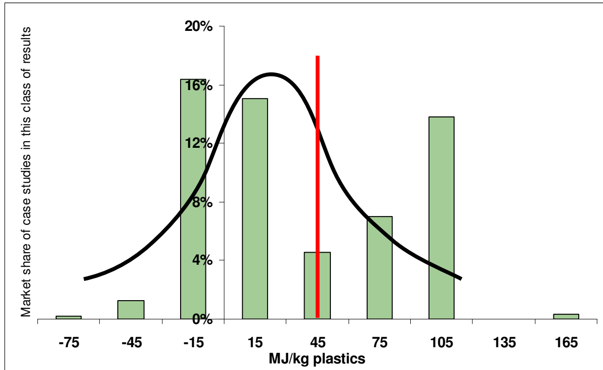
Figure 12: Results of case studies for energy savings by plastic products, aggregated into classes with a range of 30 MJ/kg each. The figure shows the sum of the market share of case studies within a certain class of result (case studies with results higher than 180 MJ/kg are not shown). The red line shows the weighted average of the case studies calculated so far (46 MJ/kg plastics). The black line shows, how an assumed average value of 23 MJ/kg plastics for the remaining amount of substitutable plastic products would relate to the results calculated so far.
