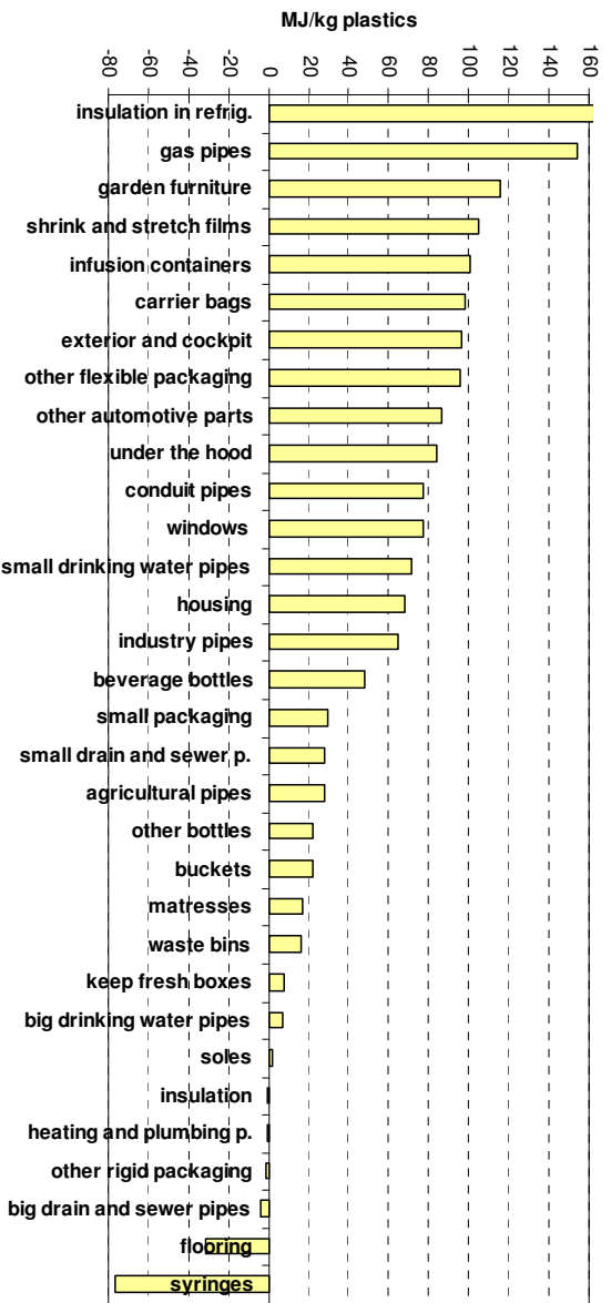
Figure 6: Energy savings of plastic products compared to alternative materials. Results in descending sorting. The value for "insulation in refrigerators" is approx. 1.800 MJ/kg PUR.
