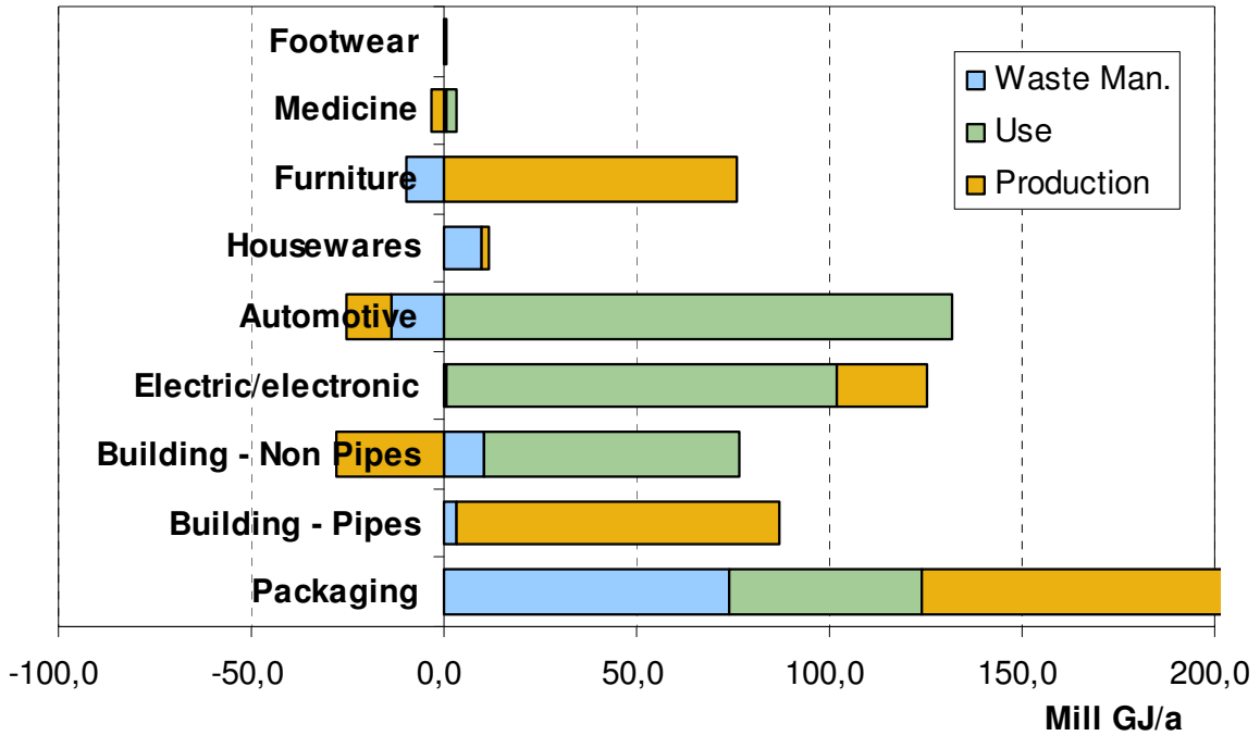
Figure 10: Energy savings (+) and additional energy demand (-) of plastic products compared to alternative materials, split into contributions of the life-cycle phases production, use and waste management. The total result for plastic packaging is 583 Mill GJ/a.
