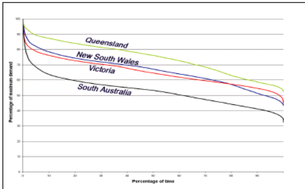
Source Figure 4: Australian annual customer load-duration shapes Kema 9 page 24
