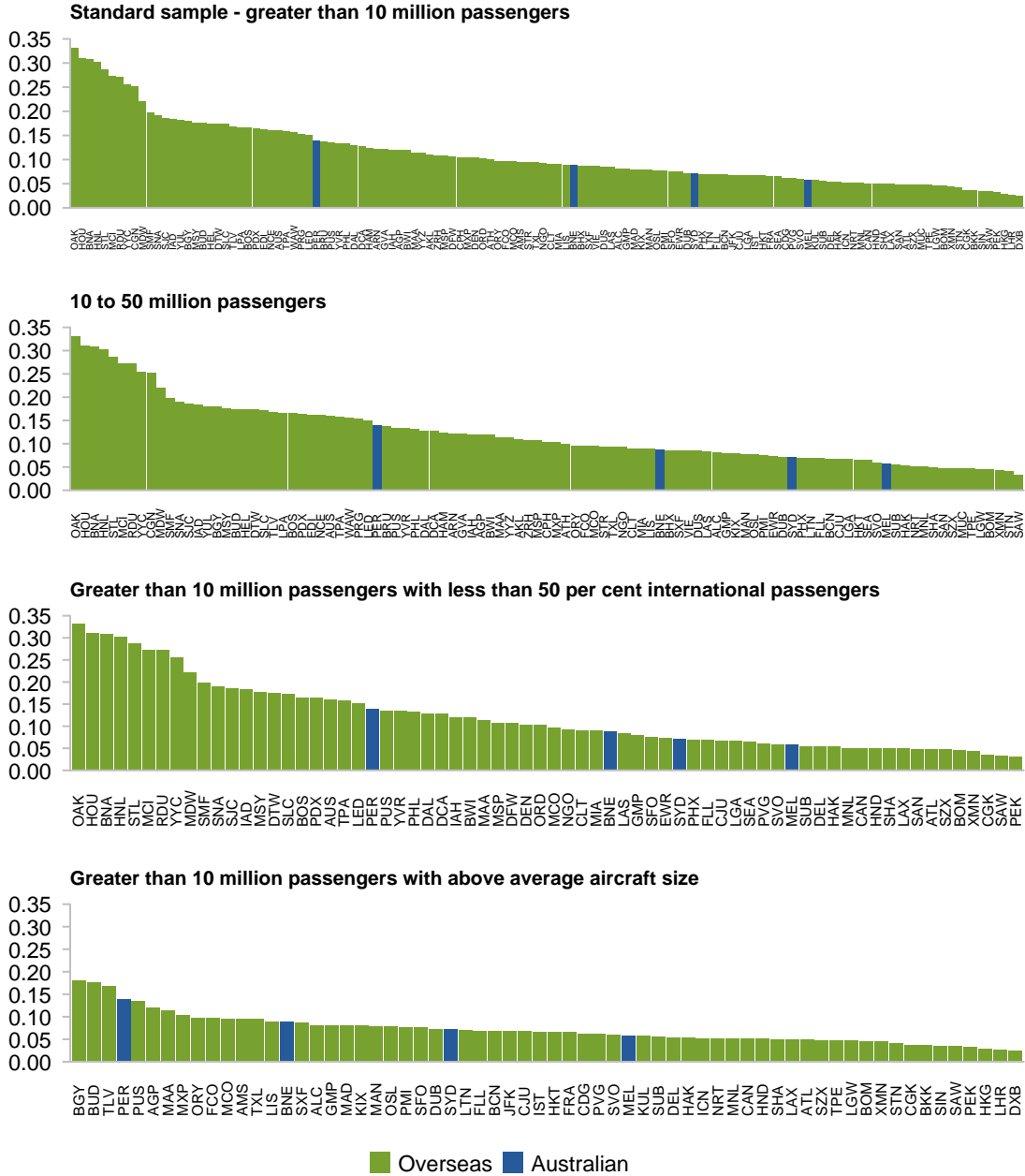
Figure B.3 Runways per million passengers a
